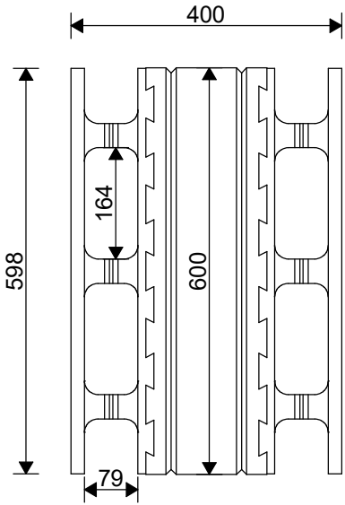
EMH-350PRO
